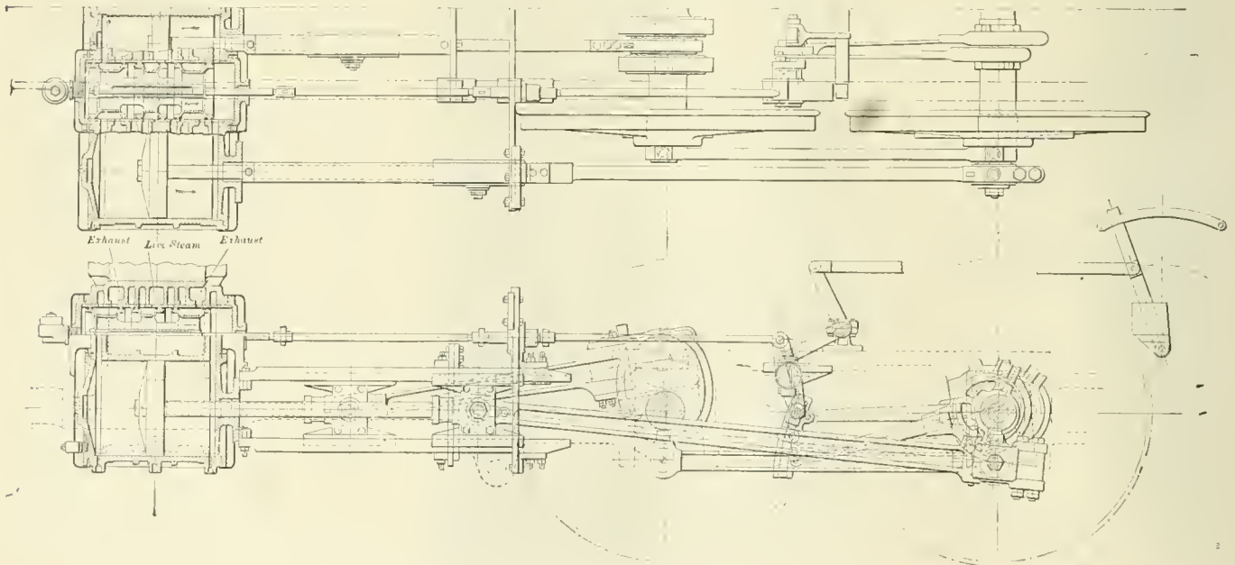
PLAN OF BALDWIN FOUR-CYLINDER BALANCED COMPOUND SHOWING CRANK AXLE.
